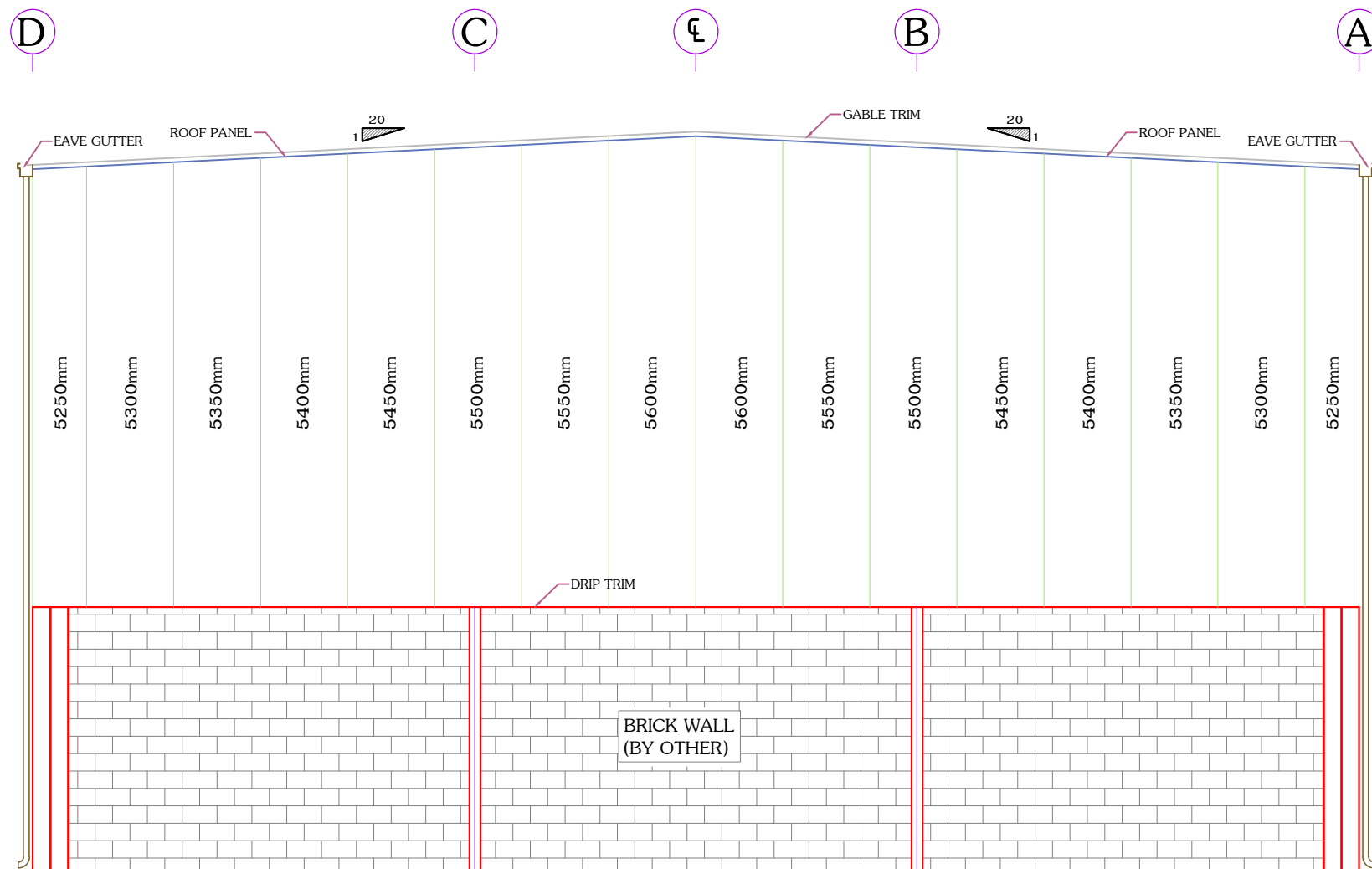
END WALL SHEETING @ GRID-5
